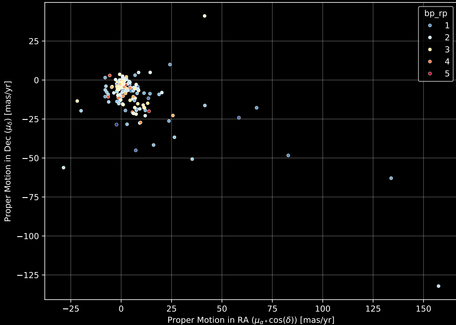
APOGEE DR17 Field: [TAUL1521] Proper Motion Diagram (n= 177)
