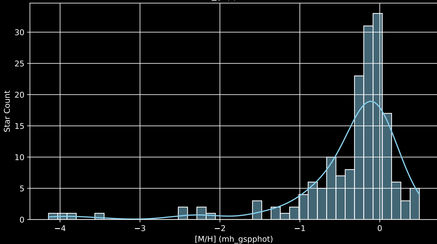
APOGEE DR17 Field: [TAUL1521 [M/H] (mh_gspphot) (n= 175)
