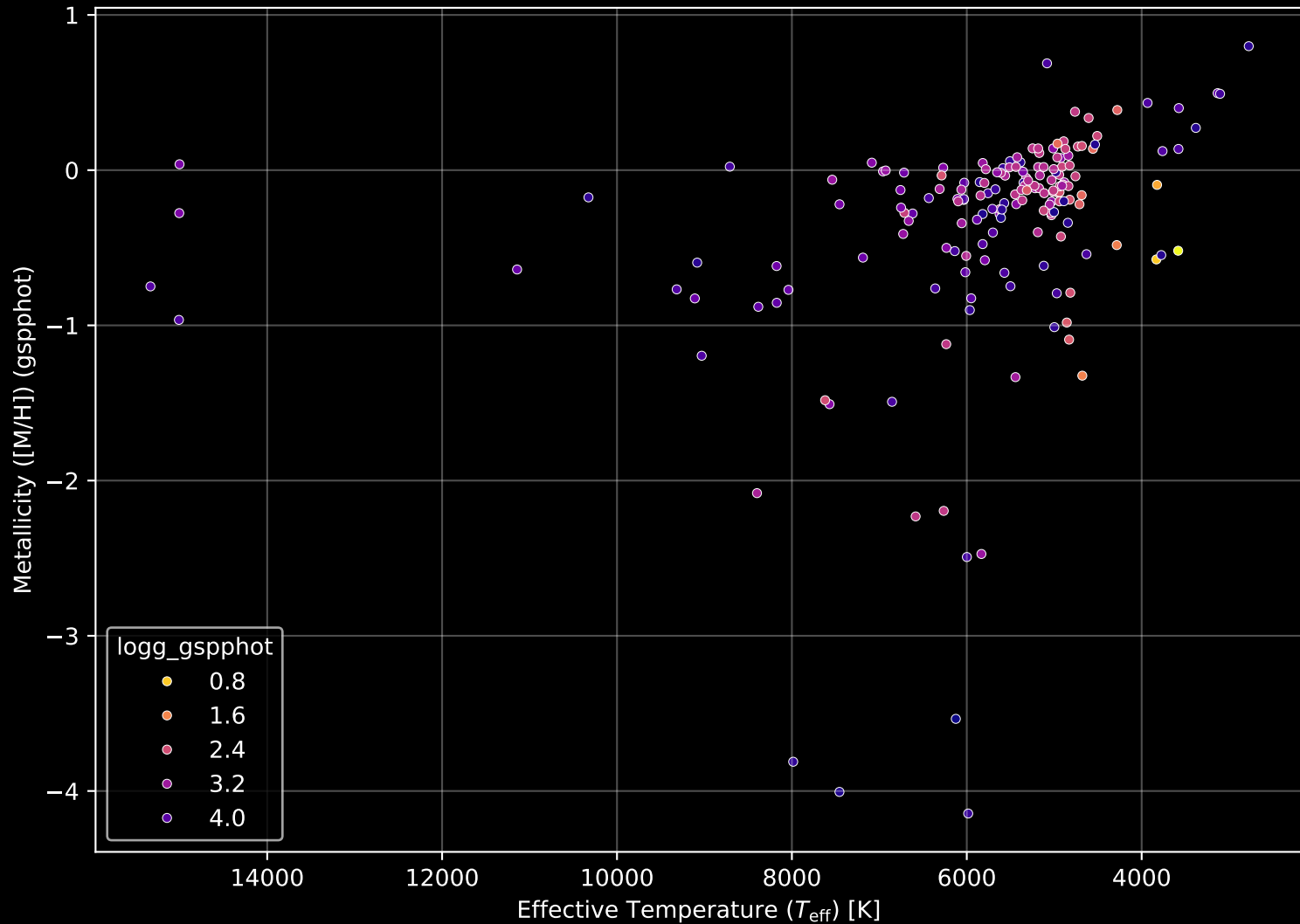
APOGEE DR17 Field: [TAUL1521] Stellar Population Parameters (n= 177)
