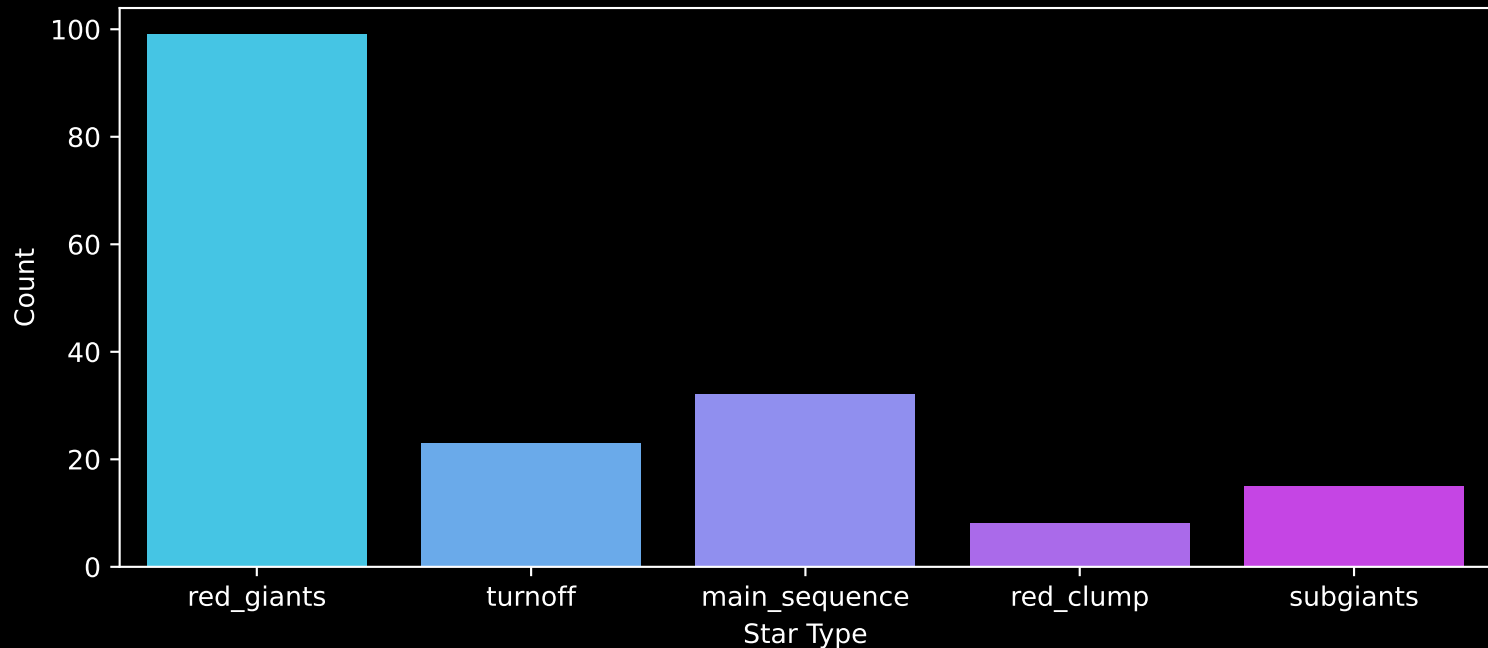
APOGEE DR17 Field: [TAUL1521] Count plot of Star Type
