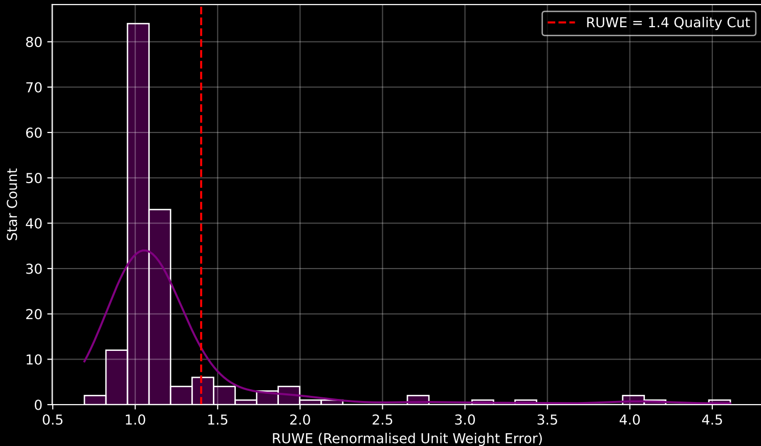
GAPOGEE DR17 Field [TAUL1521] RUWE Distribution (n= 173)
