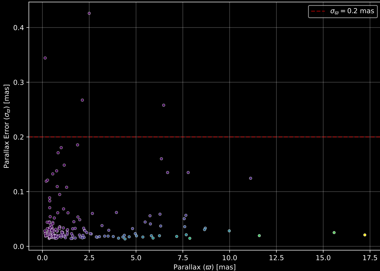
APOGEE DR17 Field: [TAUL1521] Parallax Quality (n= 177)
